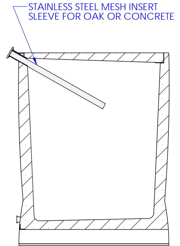
ADDITIVE INSERT
