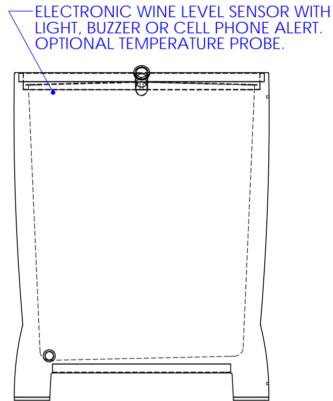
SENSOR PACKAGE
